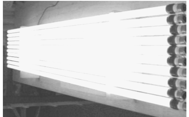
Figure 11. Photograph of lighted 10 coil-EEFL tubes in outer diameter 3.2 \times 10^{-2} m with 1.2 m long in parallel connection with single AC driving device that supplies 4 kV with 50 kHz to the electrodes of EEs.
