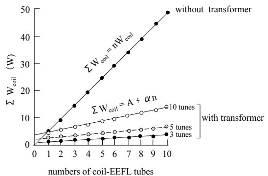
Figure 9. Total W_{coil} of 10 coil-EEFL tubes with different AC driving circuits; with and without transformer at output of voltage.
