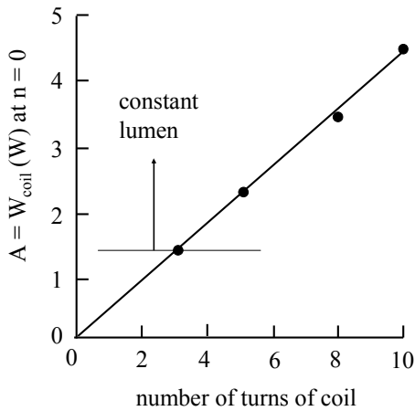
Figure 5. A-values of \Sigma W_{coil} -curves in parallel connection of coil-EEFL tubes as function of number of turning coil on coil-EEFL tube.
