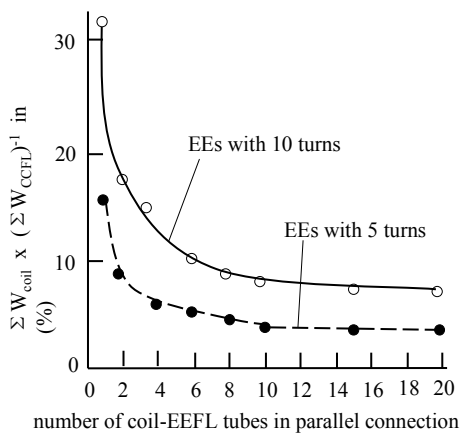
Figure 8. Experimental curve of \Sigma W_{coil} \times (\Sigma W_{CCFL})^{-1} as function of number of parallel connection of coil-EEFL tubes.
