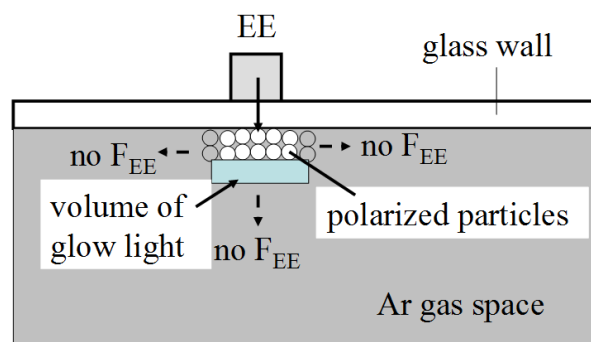
Figure 1. Illustration of anisotropic electric field, F_{EE} , from EE on glass wall of coil-EEFL tube.
